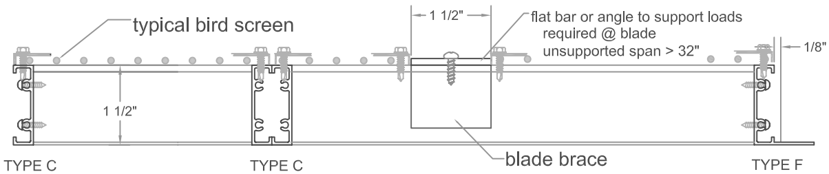
AA - ACTIVE MODEL SECTIONS
