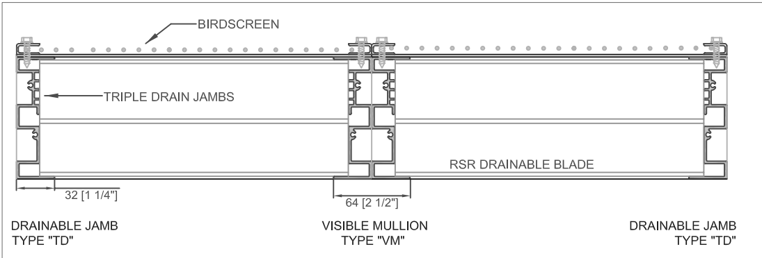
BB - TYPICAL HORIZONTAL SECTION
