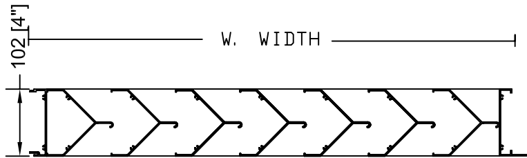
SECTION C JAMB MULLION TYPE C FRAME
